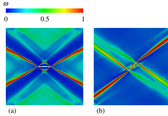
Figure 9: Localization of damage, parameter \omega defined by Eq. (15), in a specimen subject to tensile stretching with an embedded rigid line inclusion inclined at angles \bar{\theta} = 0^\circ (a) and \bar{\theta} = 45^\circ (b) with respect to the horizontal axis. Shear bands exhibit a double symmetry in (a), while the shear bands closer to the inclusion axis are the most intense in (b).
