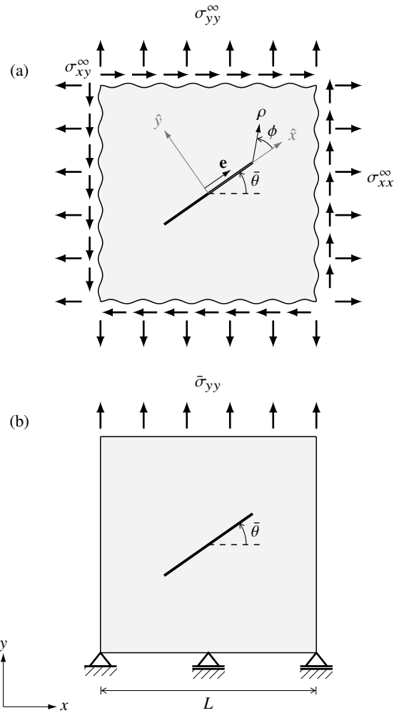
Figure 2: The two elastic boundary value problems used for the validation of the numerical model: (a) One RLI is embedded in an infinite elastic domain, and (b) the same RLI lies within a square domain of side L . The analytical solution of the elastic boundary value problem in panel (a) is used to validate the numerical model applied to the boundary value problem in panel (b). The unit vector \mathbf{e} = \{\cos \bar{\theta}, \sin \bar{\theta}\} is aligned parallel to the inclusion line.
