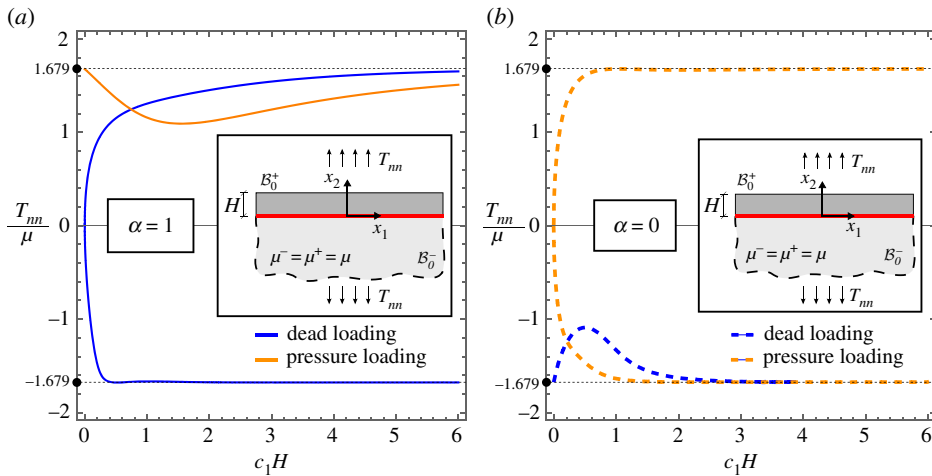
Figure 4. Bifurcation of a layer connected to an elastic incompressible half-space through a sliding interface. Both layer and half-space are modelled with the same neo-Hookean material and subject to the same prestress orthogonal to the interface. Both dead and pressure loadings are considered for the two interfacial conditions \alpha = 1 and \alpha = 0 (the latter condition is incorrect and included only for comparison). The normalized bifurcation stress T_{nn}/\mu is reported versus the normalized wavenumber of the bifurcated field c_1H . Note that for dead load bifurcation in tension is possible only when the correct interfacial condition, \alpha = 1 , is considered. (Online version in colour.)
