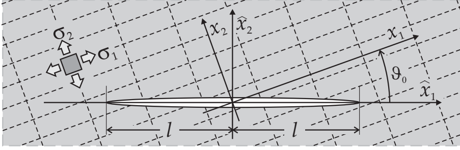
Figure 2: Finite-length ( 2l ) crack in a prestressed, orthotropic material inclined at an angle \vartheta_0 (positive when anticlockwise) with respect to the orthotropy axes x_1 and x_2 .
